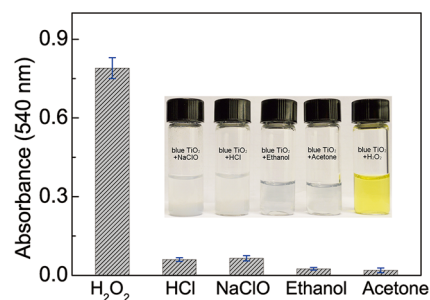
Figure 4. Selectivity analysis for H 2 O 2 detection by monitoring the relative absorbance. Inset: the analyte concentrations are as follows: 1 M sodium hypochlorite (NaClO), 2 M hydrochloric acid (HCl), 1 M ethanol, 1 M acetone, 0.5 M hydrogen peroxide (H 2 O 2 ). Error bar: standard deviation.
