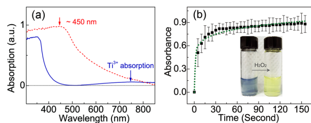
Figure 2. (a) Typical absorption spectra of TiO 2 :Ti 3+ before (solid line) and after (dashed line) adding of H 2 O 2 . (b) Typical absorbance kinetic of TiO 2 :Ti 3+ NPs and H 2 O 2 at 450 nm. Inset shows schematic images of TiO 2 :Ti 3+ NPs without (left) and with (right) adding of H 2 O 2 solution. Error bar: standard deviation.
