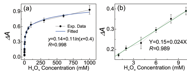
Figure 3. (a) Relationship between absolute absorbance \Delta A at 450 nm and concentration of H 2 O 2 over a range between 1 \times 10^{-6} and 1 M. The blue solid line is the fitted curve. (b) Linear fitting of absolute absorbance at 450 nm versus H 2 O 2 concentration over a range between 1 and 10 mM. Error bar: standard deviation.
