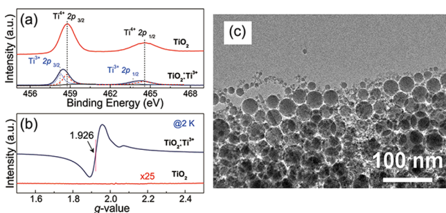
Figure 1. (a) Ti 2p XPS spectra and (b) EPR spectra at 2 K for rutile TiO 2 before and after 355 nm laser irradiation; (c) TEM of TiO 2 :Ti 3+ NPs.
